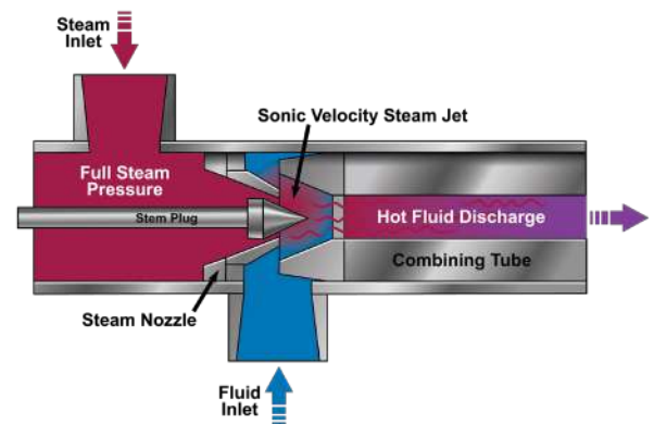
Figure 3: Internally Modulated direct-contact steam heating
