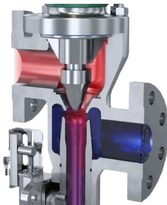
Figure 1: Hydroheater technology injects precise amounts of steam into the process fluid
