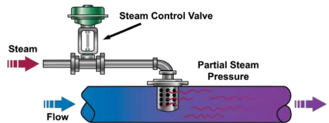
Figure 2: External Modulated direct-contact steam heating
